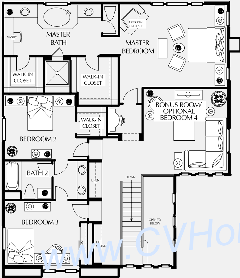
PLAN 2CR SECOND STORY
