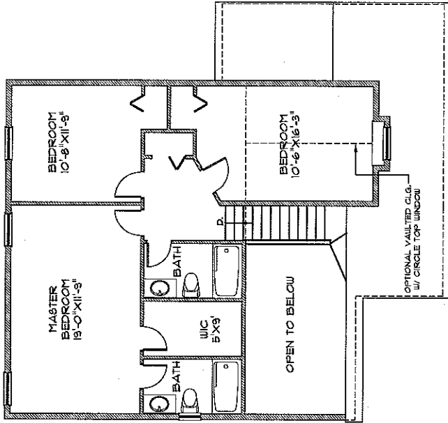
2ND FLOOR OPT 2
