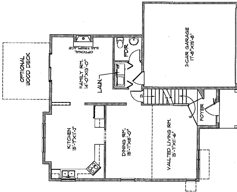
FIRST FLOOR OPT 2 ADDING 15 SQ. FT. @ KITCHEN
