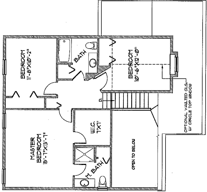
2ND FLOOR OPT 1 - 810 S.F.
