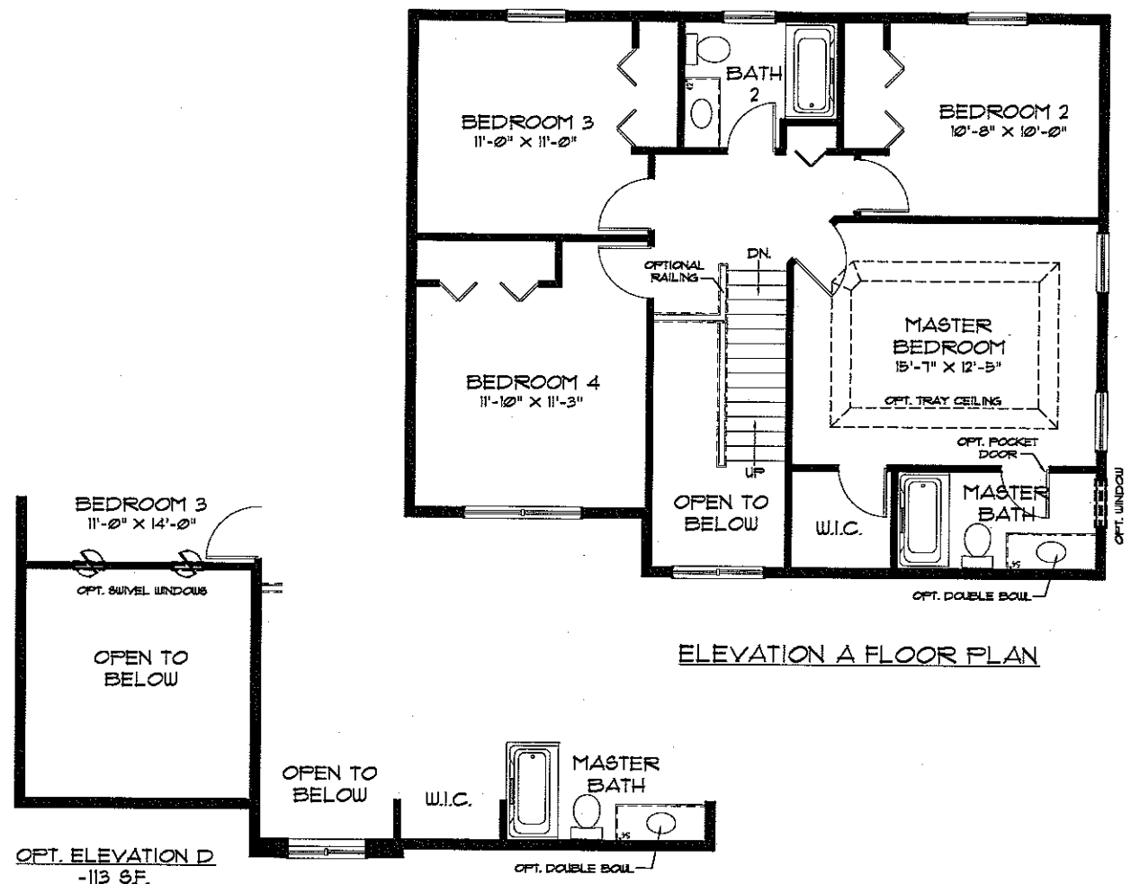
SECOND FLOOR
