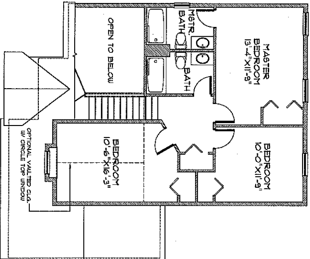
2ND FLOOR OPT 2
