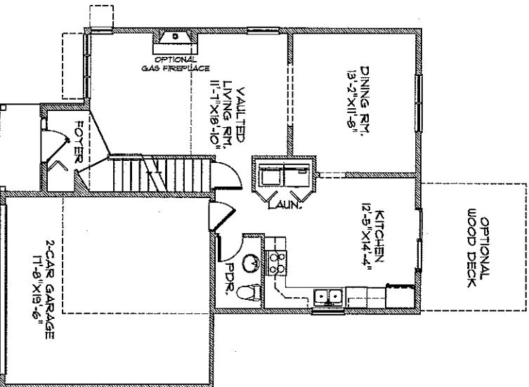
FIRST FLOOR OPT 1 - 166 S.F.
