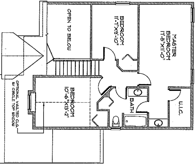
2ND FLOOR OPT 1 - 728 S.F.
