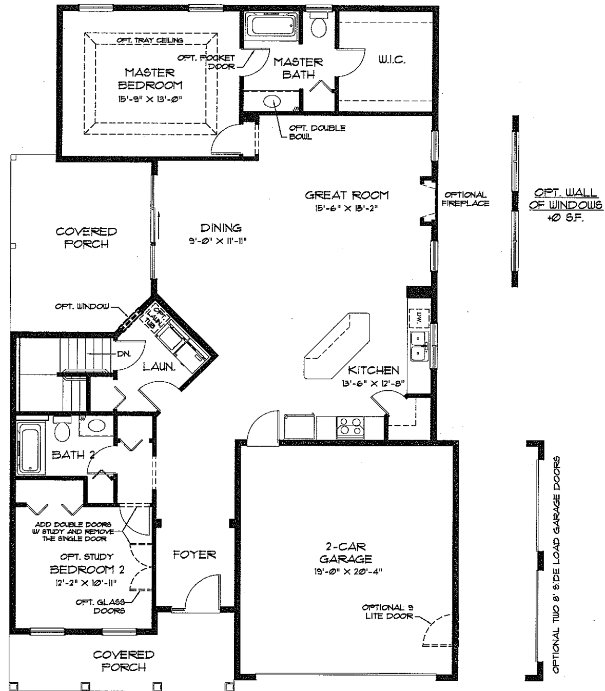
ELEVATION A FLOOR PLAN
